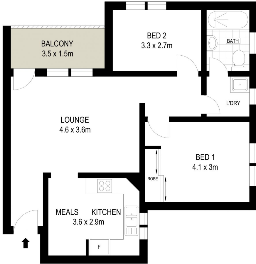
LEVEL ONE
