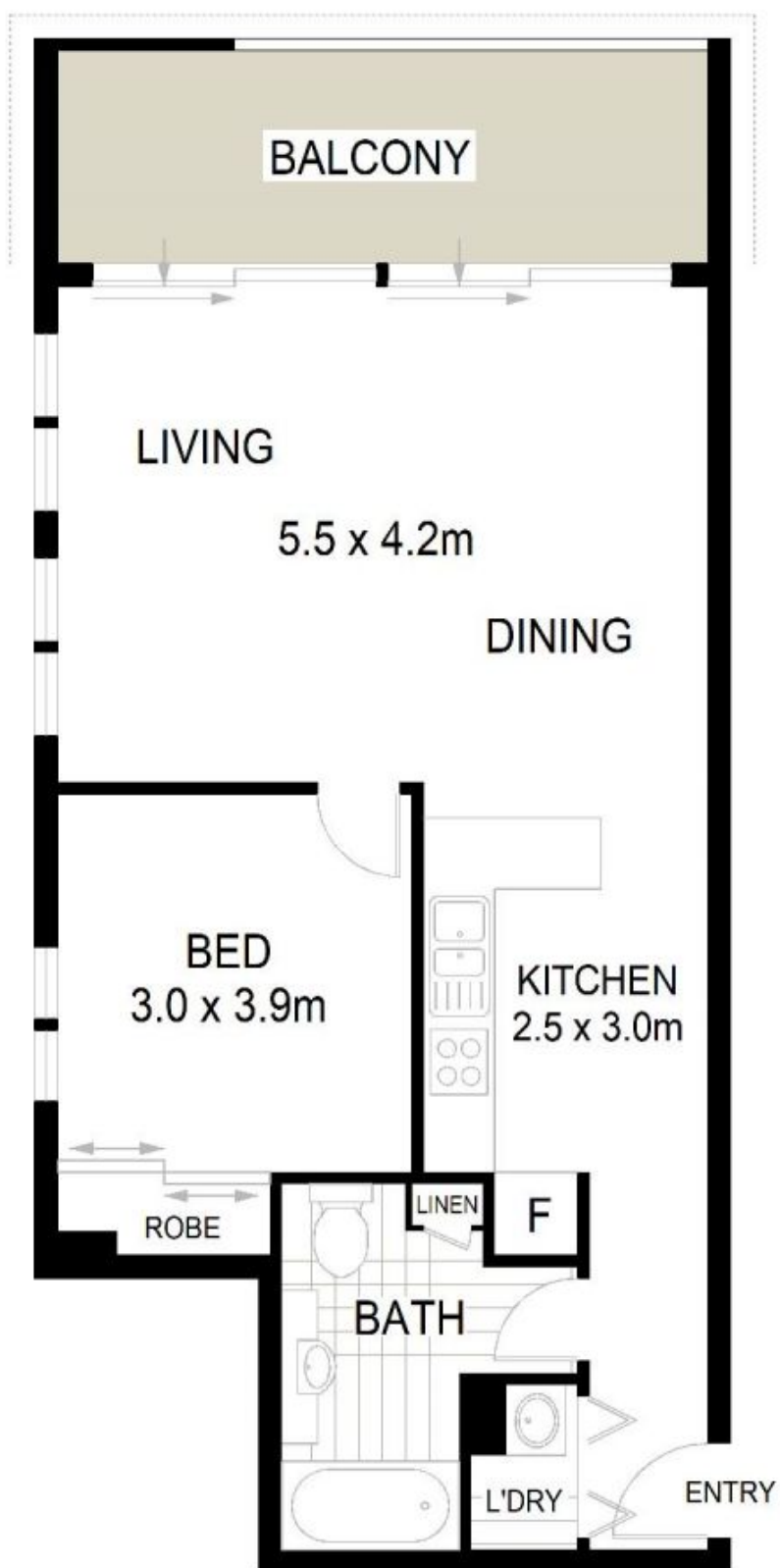
LEVEL TWO
