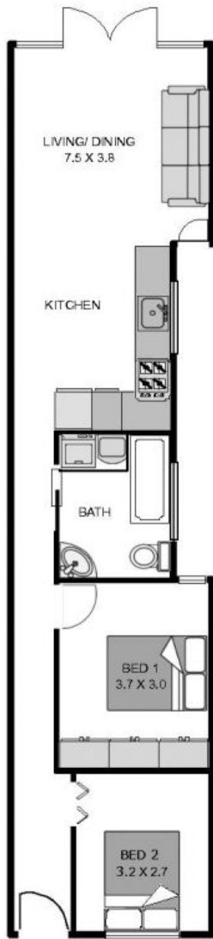
FLOOR PLAN
