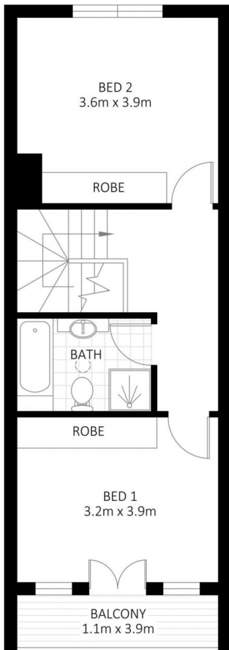
UPPER FLOOR
