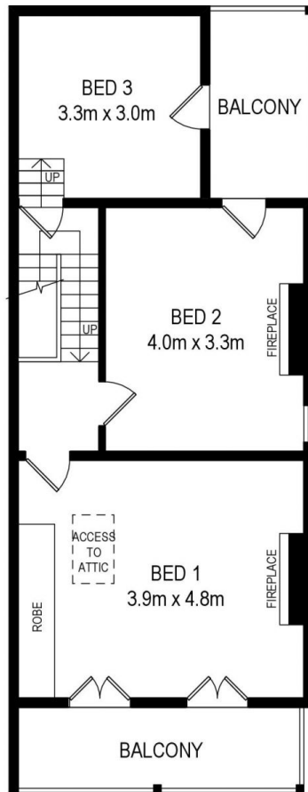
UPPER LEVEL
