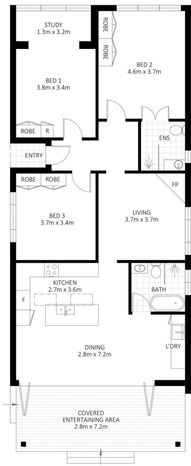
FLOOR PLAN
