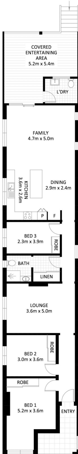
FLOOR PLAN
