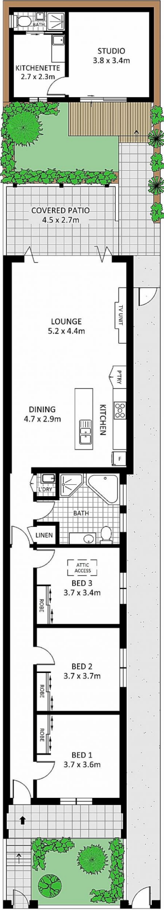
FLOOR PLAN
