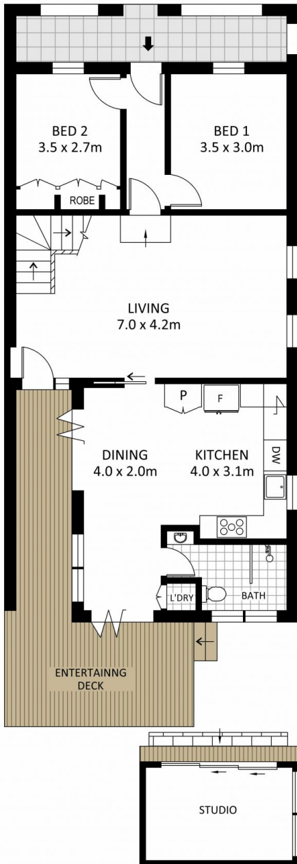
FLOOR PLAN
