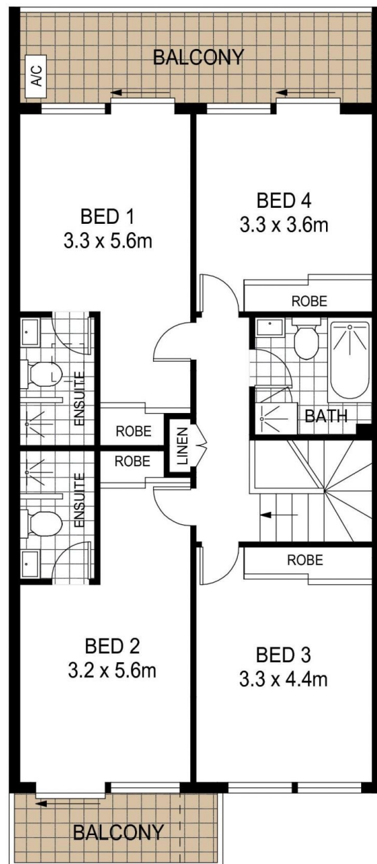
LEVEL ONE
