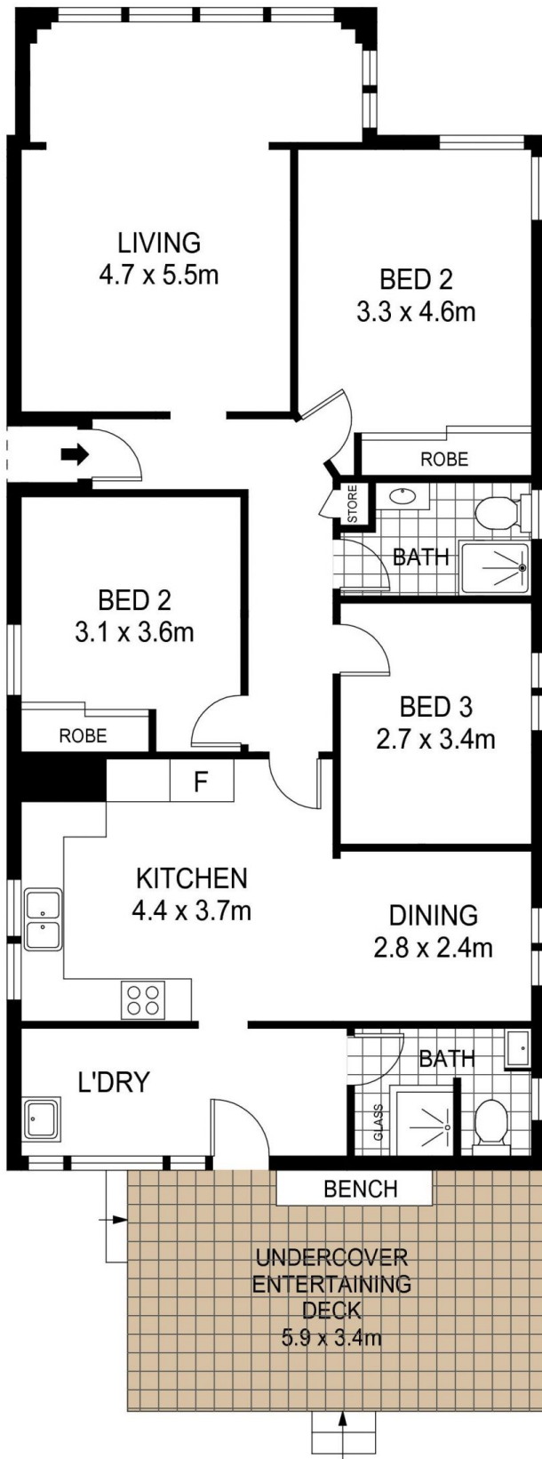
GROUND LEVEL
